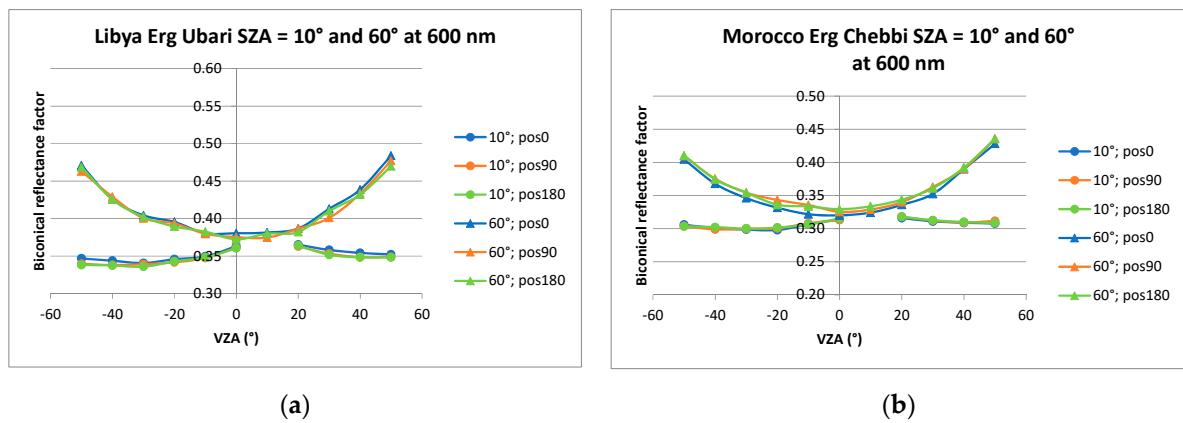
Figure 13. BCRF for the minimum (10°) and the maximum (60°) solar zenith angles, in the principal plane, for: (a) Libya; (b) Morocco.
