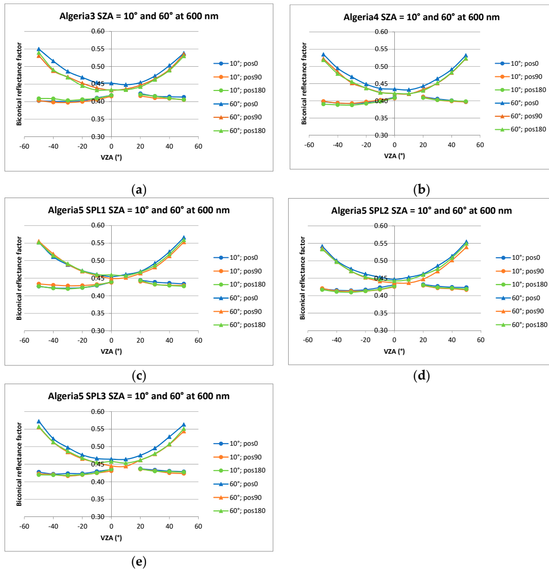
Figure 11. BCRF for the minimum (10°) and the maximum (60°) solar zenith angles, in the principal plane, for Algerian samples: (a) Algeria3;(b) Algeria4; (c) Algeria5 sample 1; (d) Algeria5 sample 2; (e) Algeria5 sample 3.
