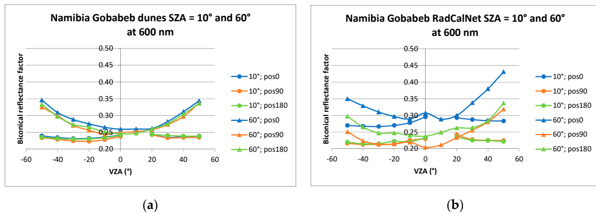
Figure 14. BCRF for the minimum ( 10^\circ ) and the maximum ( 60^\circ ) solar zenith angles, in the principal plane, for Namibian sites near Gobabeb: (a) dunes; (b) RadCalNet.
