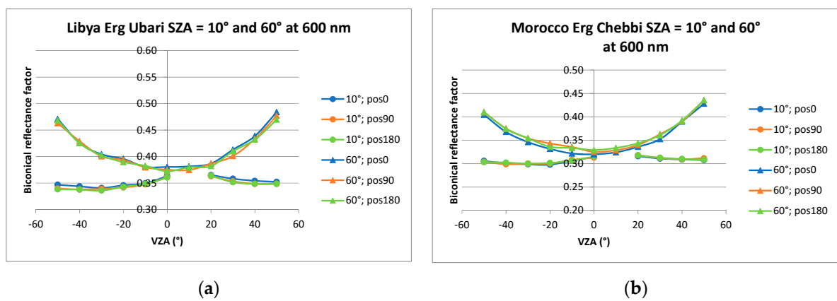
Figure 13. BCRF for the minimum (10°) and the maximum (60°) solar zenith angles, in the principal plane, for: (a) Libya; (b) Morocco.
