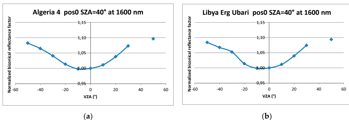
Figure 20. Normalized BCRF for Algeria4 (a) and Libya Erg Ubari (b) in the principal plane.
