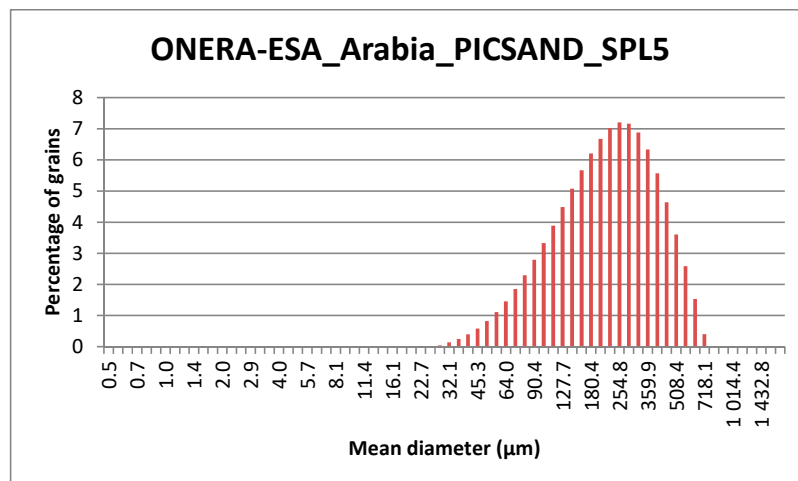
Figure 18. Grain size distribution for the Arabia_PICSAND_SPL5 sample.
