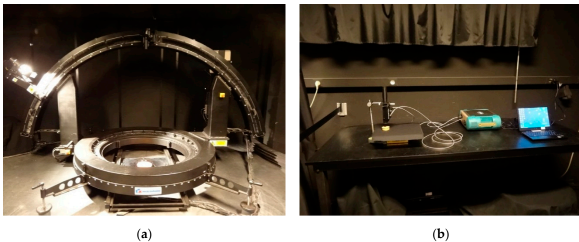
Figure 1. Measurement devices: (a) ONERA BCRF measurement device named “Banc de BRDF grands échantillons”; (b) 1 geometry BCRF measurement set up using a contact probe.
