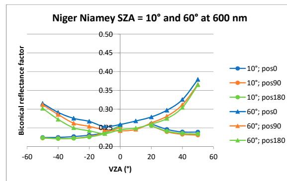
Figure 15. BCRF for the minimum ( 10^\circ ) and the maximum ( 60^\circ ) solar zenith angles, in the principal plane, for Nigerian site near Niamey.
