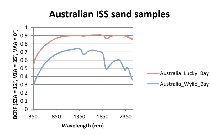
Figure 10. Spectral variation of BCRF for the Australian Internal Soil Standard (ISS) samples.
