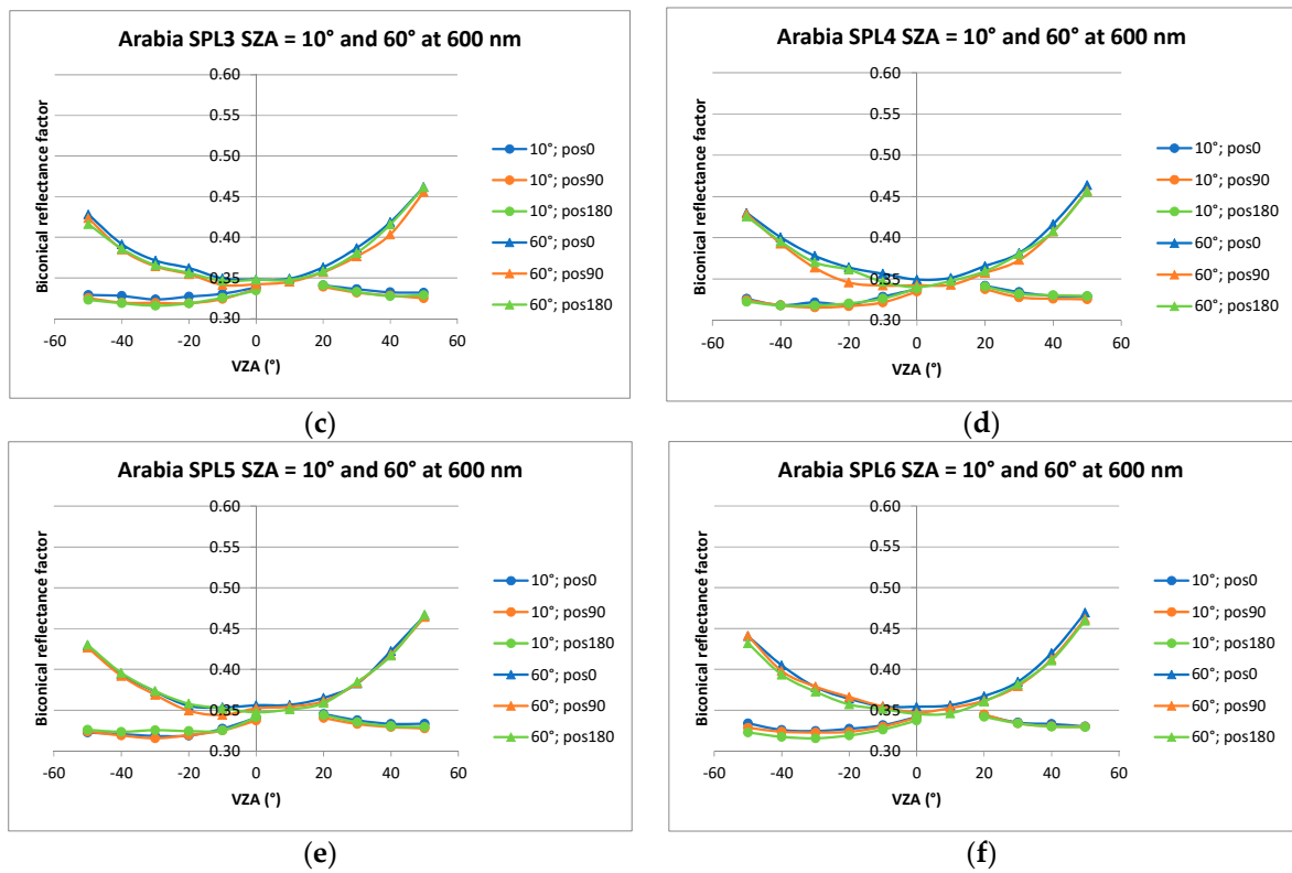
Figure 12. BCRF for the minimum (10°) and the maximum (60°) solar zenith angles, in the principal plane, for Arabian samples: (a) sample 1; (b) sample 2; (c) sample 3; (d) sample 4; (e) sample 5; (f) sample 6.
