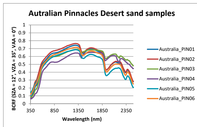
Figure 7. Spectral variation of BCRF for the Australian Pinnacles Desert sand samples.
