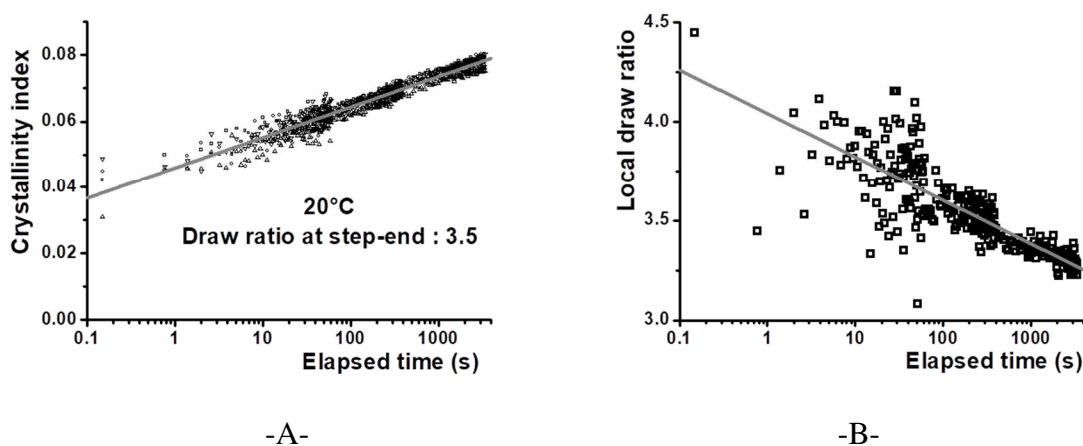
Figure 12. Time-dependence of –A the crystallinity index; all four investigated samples are reported to illustrate the data dispersion; the grey line is a linear adjustment. B- the local draw ratio as computed from \langle P_2^{RX} \rangle . Each point corresponds to an average on the four investigated samples (20°C; elongation at step-end: 3.5).
