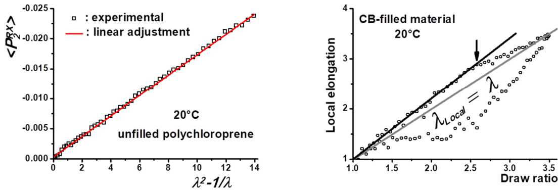
Figure 4. A- Elongation-dependence of the coefficient \langle P_2^{RX} \rangle for the unfilled material before SIC onset (each point in an average over 12 samples). B- Local elongation versus applied elongation for the CB-filled material (each point in an average over 13 samples). The vertical arrow in B indicates the onset of relaxation of the local elongation.
