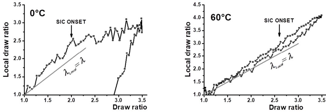
Figure 6. A- Elongation-dependence of the local draw ratio for two representative temperatures.
