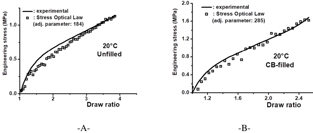
Figure 8. Adjustment of the engineering stress before SIC onset by the stress optical law for A- the unfilled material, B- The CB-filled material.
