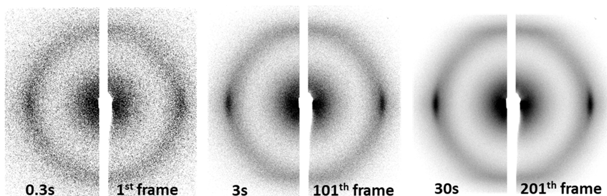
Figure 11. Diffraction patterns collected during a tensile test sequence with increasing acquisition durations (elongation at step-end: 3.5; temperature: 20°C)
