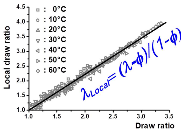
Figure 7. Draw ratio -dependence for the local draw ratio before SIC onset as measured on the tested temperature range. Each data point is an average for a minimum of two samples from the same batch.
