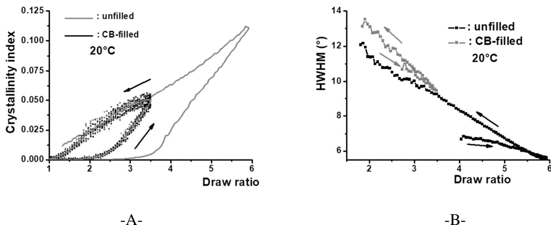
Figure 2. Comparison for CB-filled and unfilled samples of the draw ratio -dependence of A- the crystallinity index; the solid gray line on top of experimental points for the CB-filled material visualizes the average over the 13 studied samples (black points). B- the half-width at half-maximum for the crystalline diffraction peak.
