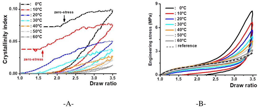
Figure 5. Effect of temperature on A- the crystallinity index, B- the stress-strain curve during mechanical cycling (each curve is an average for two samples from the same batch).
