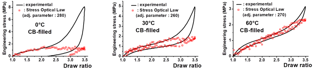
Figure 9. Contribution of the amorphous fraction to stress as derived from the stress optical law at three representative temperatures.
