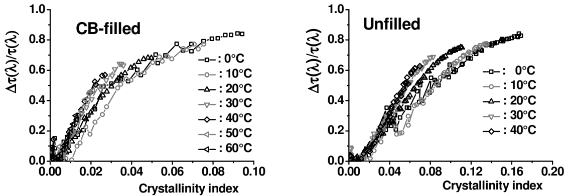
Figure 10. Contribution to the total engineering stress of the stress fraction linked to SIC.
