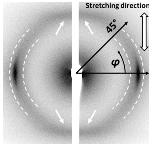
Figure 1. Representative diffraction pattern of a partially strain-crystallized CB-filled CR sample (draw ratio: 3.5; 0°C; exposure time: 10s). The blind central vertical line corresponds to the gap between the two detecting elements of the X-ray camera.
