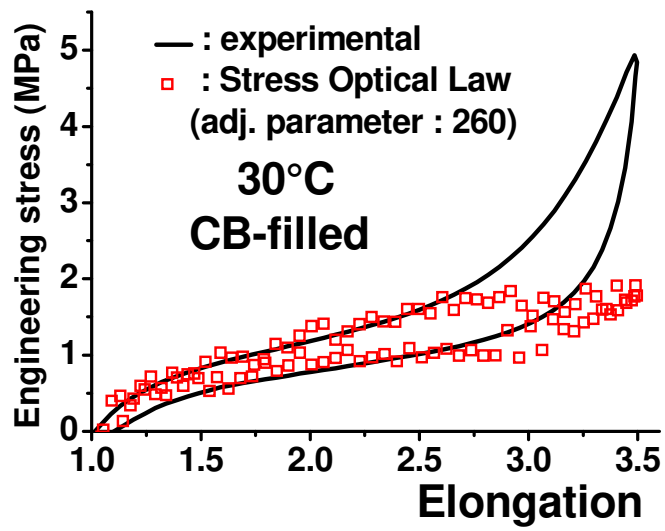
Contribution of the amorphous fraction to stress in carbon black filled polychloroprene at 30°C
