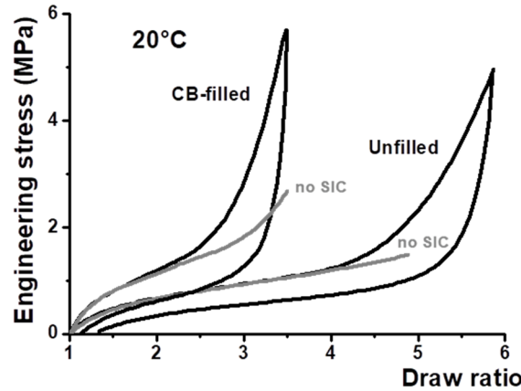
Figure 3. Stress-strain curves for CB-filled and unfilled samples.
