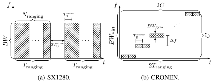
Fig. 5. Spectrum occupation for the two-way ranging protocols.
