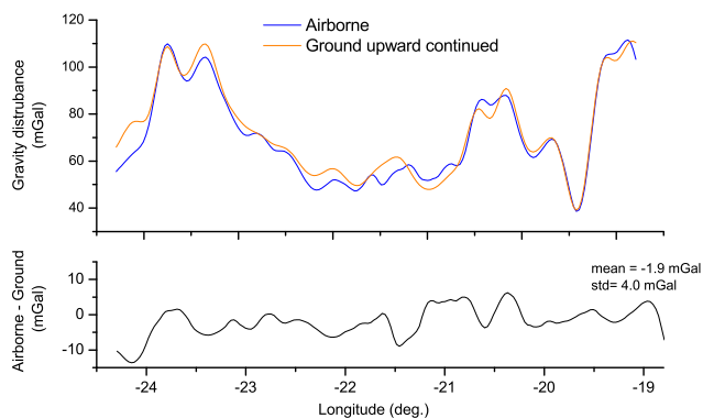
Fig. 8 Comparison between airborne measurements (average of forward and backward) and ground measurements upward continued along the line Akureyri-Snæfellsjökull
