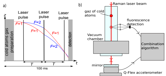
Fig. 1 Principle of the atom accelerometer. a) Temporal sequence. b) Set-up of the atom accelerometer.
