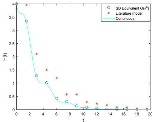
Fig. 5.2. Evolution of the energy with \alpha = 0.4, \delta = 1.5 .
