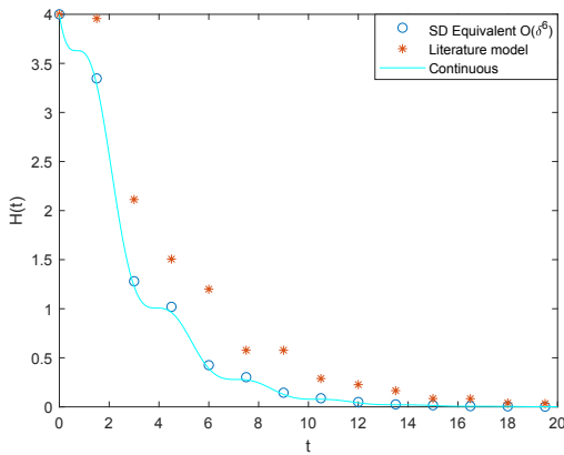
Fig. 5.2. Evolution of the energy with \alpha = 0.4, \delta = 1.5 .
