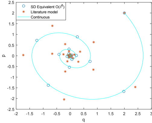
Fig. 5.1. Evolution of the system with \alpha = 0.4, \delta = 1.5 .
