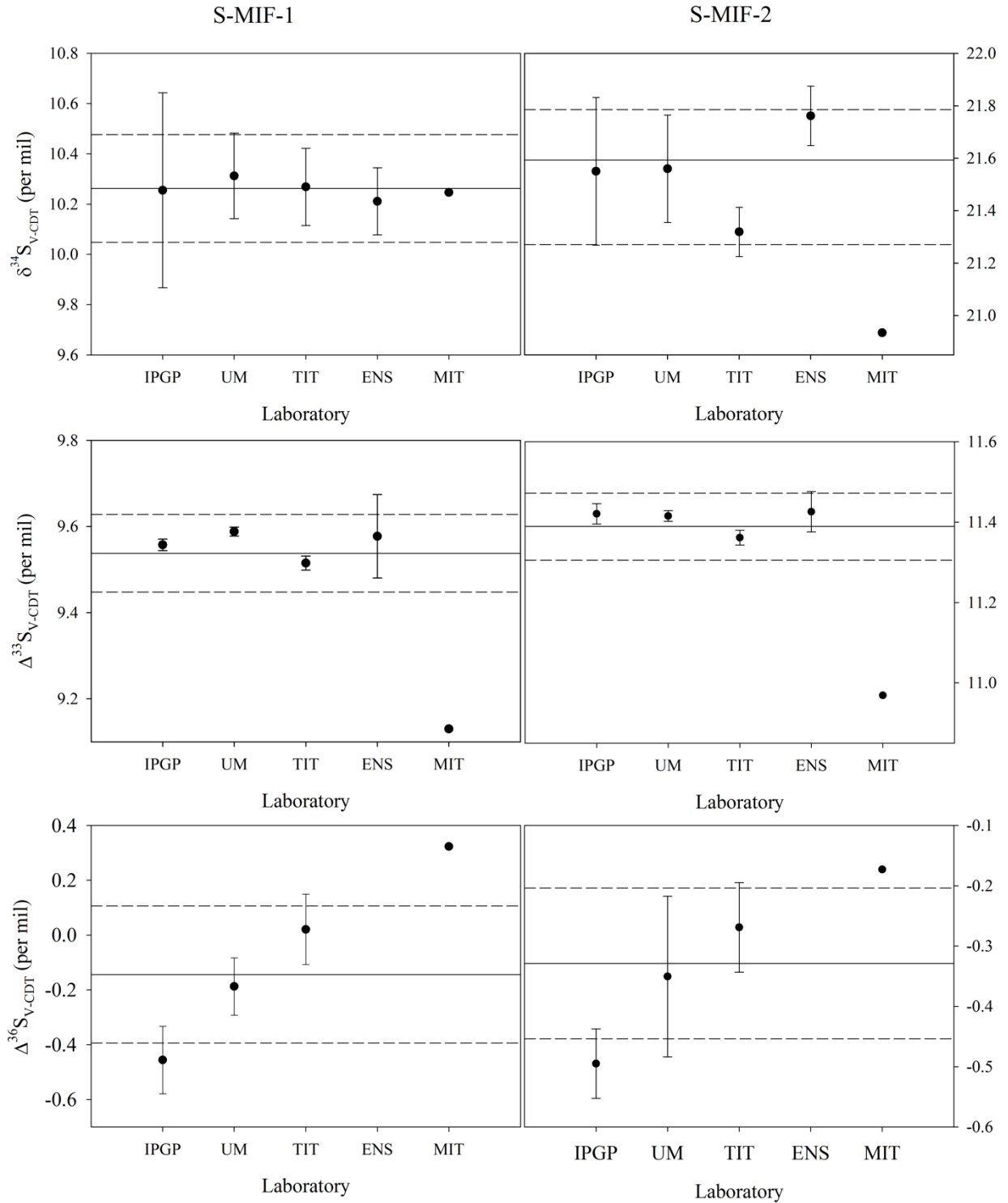
Figure 1. The individual laboratory results of S-MIF-1 and S-MIF-2. The error bars for the individual laboratory results are 1 \sigma ; The Solid and dashed lines represent the interlaboratory averages and \pm 1 \sigma , respectively.
