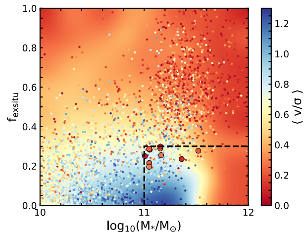
Figure 1. 2D histogram showing the fraction of ex situ mass versus stellar mass of galaxies in the Horizon-AGN simulation at z = 0.06 . The individual points show a random selection of galaxies and the background colour is derived using a cubic spline interpolation over all galaxies. The colour coding indicates the value of \frac{V}{\sigma} of both the background and the individual points. Massive spheroids typically exhibit large fractions of ex situ stellar mass. The spheroids in this study have \frac{V}{\sigma} < 0.3 , f_{ex\ situ} < 0.3 , and stellar mass > 10^{11} M_\odot , and are shown using the large outlined points in the bottom right-hand corner of the plot. Note that we do not consider objects that may have \frac{V}{\sigma} < 0.3 but are in ongoing mergers, as the \frac{V}{\sigma} values of such objects are highly transient and the morphology of the remnant is uncertain.
