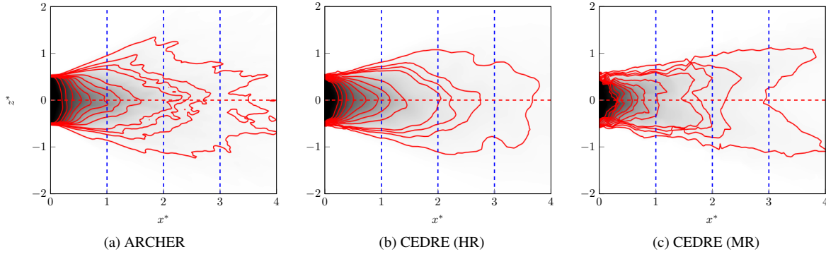
Fig. 9: Averaged liquid volume fraction isolines \langle \alpha_l \rangle_t = 0.1 to 1 , dashed located at x^* \in \{d_l, 2d_l, 3d_l\} and y^* = 0 . Reader must take care to the fact that the \langle \alpha_l \rangle_t range is different for the three slices.
