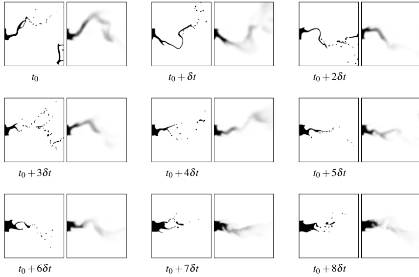
Fig. 7: Time lapse of liquid volume fraction near the injector (ARCHER), \alpha_l = 0 . Left: ARCHER, right: CEDRE. We define t_0 as the starting time and \delta t as the time step.
