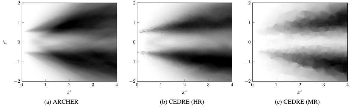
Fig. 17: Longitudinal Reynolds stress tensor component \langle v'_x v'_x \rangle_t . \langle v'_x v'_x \rangle_t \in [0 m^2/s^2, 300 m^2/s^2]
