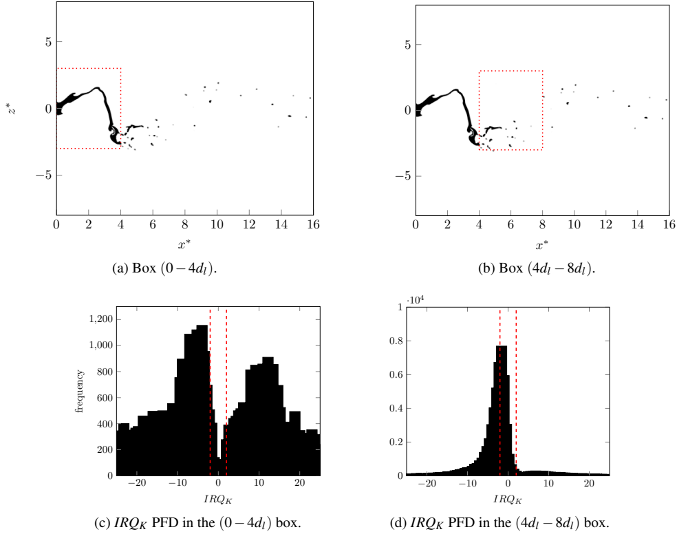
Fig. 6: IRQ_k PDF analysis at time t = 12\text{ ms} (bottom), in two regions identified by the red dashed rectangles drawn on the plan y^* = 0 showing liquid volume fraction \alpha_l (top).
