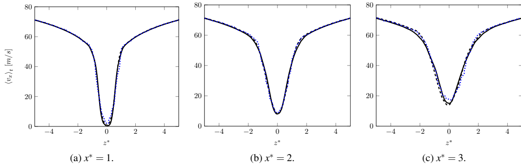
Fig. 14: Averaged axial velocity \langle v_x \rangle_t along Figure 9 dashed lines. — ARCHER, - - - CEDRE (HR), ···· CEDRE (MR).
