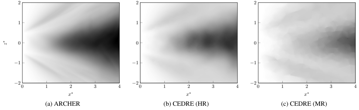
Fig. 15: Transverse Reynolds stress tensor component \langle v'_z v'_z \rangle_t = 0 \rightarrow 350 m^2/s^2 at y^* = 0 .
