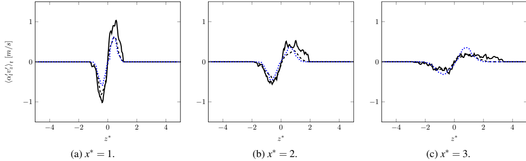
Fig. 20: Transversal liquid flux tensor component \langle \alpha'_l v'_z \rangle_t along Figure 9 dashed lines. — ARCHER, - - - CEDRE (HR), ···· CEDRE (MR).
