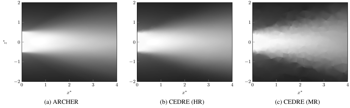
Fig. 13: Averaged axial velocity \langle v_x \rangle_t = 0 to 70 \text{ m/s} at y^* = 0 .
