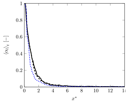
Fig. 8: Averaged liquid volume fraction \langle \alpha \rangle_t along streamwise axis. — ARCHER, - - - CEDRE (HR), ···· CEDRE (MR).
