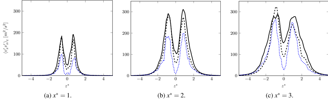
Fig. 18: Longitudinal Reynolds stress tensor component \langle v'_x v'_x \rangle_t along Figure 9 dashed lines. — ARCHER, - - - CEDRE (HR), ···· CEDRE (MR).
