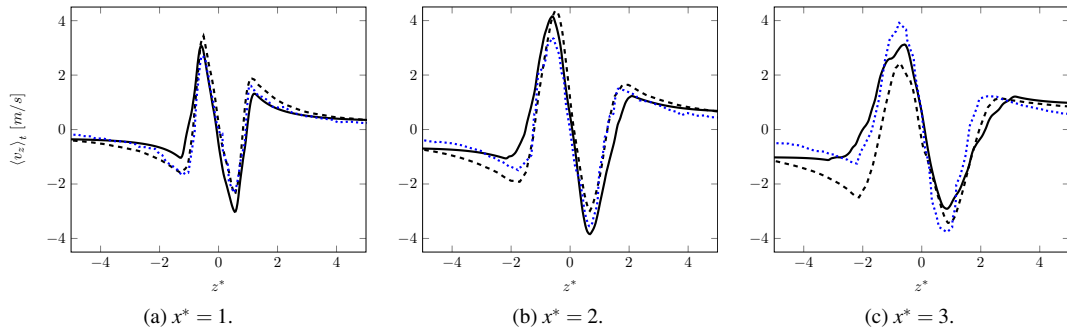
Fig. 12: Averaged transverse velocity \langle v_z \rangle_t along Figure 9 dashed lines. — ARCHER, - - - CEDRE (HR), ···· CEDRE (MR).
