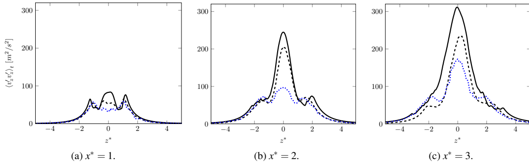
Fig. 16: Transverse Reynolds stress tensor component \langle v'_z v'_z \rangle_t along Figure 9 dashed lines. — ARCHER, ---- CEDRE (HR), ..... CEDRE (MR).
