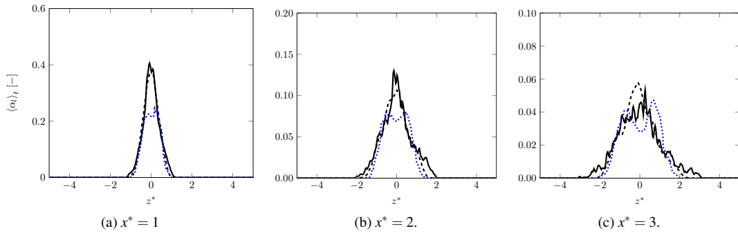
Fig. 10: Averaged liquid volume fraction \langle \alpha_l \rangle_t along Figure 9 dashed lines. — ARCHER, - - - CEDRE (HR), ···· CEDRE (MR).
