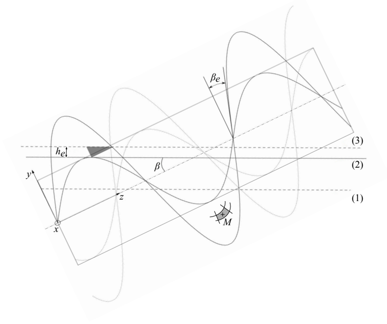
Figure 3 Archimedean screw profile in the system (O, x, y, z)
