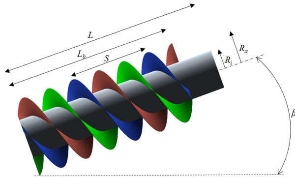
Figure 1 Geometrical parameters of the screw
