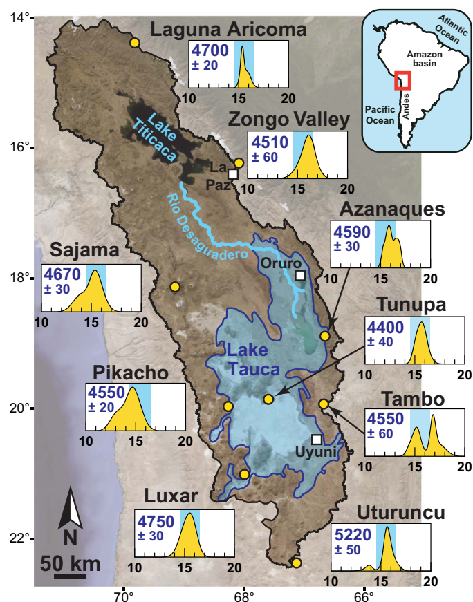
Fig. 2. Map of the Altiplano basin showing locations of the nine paleoglacioclated sites and associated geochronological constraints ( ^3\text{He} and ^{10}\text{Be} dating in thousand years BP) and ELA (in meters above sea level). CRE ages (presented in age probability density function plots) at each site (yellow points) constrain the extent of glacier cover coeval with the Taucá highstand (16.5 to 14.5 ka BP, above 3760 m, dark blue contour on the map, and vertical blue bands on the age plots). The horizontal axis of each graph shows the CRE age (in thousand years before 2010). The blue number in each age plot is the associated ELA in meters above sea level (see the Supplementary Materials)
