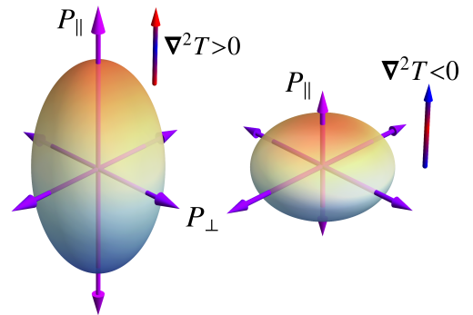
Figure 2: Illustration of the anomaly-induced asymmetry (47) between the pressure components in the transverse plane ( P_{\perp} ) and in the longitudinal directions ( P_{\parallel} ) along the temperature inhomogeneities T = T(x_{\parallel}) (the dimensions illustrate the strength of the components of the pressure and not the geometry of the system).
