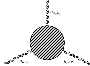
Figure 1: The 1PI diagram for the TTT vertex (39).
