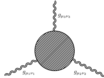
Figure 1: The 1PI diagram for the TTT vertex (39).
