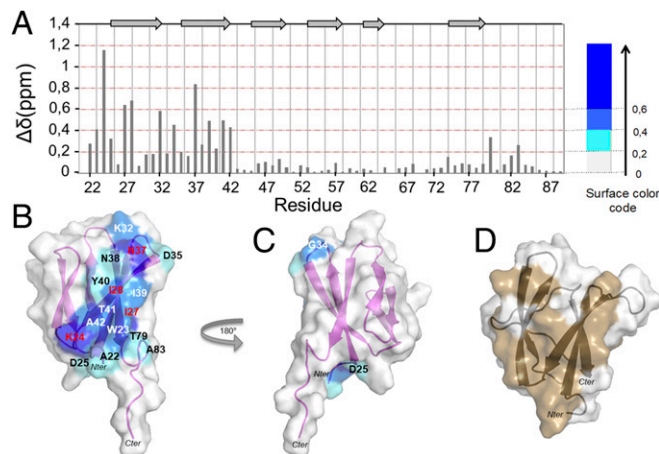
Fig. 3. AVR1-CO39 binds RGA5 HMA through the interface defined by the crystal structure of the complex. (A) Plot of the chemical shift differences ( \Delta\delta (ppm)) between unbound ( R = 0 ) and RGA5 HMA -bound dSP-AVR1-CO39 ( R = 2 ). Chemical shift differences were calculated as the Hamming distance (31), \Delta\delta (ppm) = |\Delta\delta(^1\text{H})_{ij}| + 0.102 \times |\Delta\delta(^{15}\text{N})_{ij}| , where \Delta\delta(^1\text{H})_{ij} and \Delta\delta(^{15}\text{N})_{ij} are the differences of the 1 H and 15 N chemical shifts at R = 0 and R = 2 , respectively. (B) Structure of dSP-AVR1-CO39 showing the chemical shift differences from NMR titration with the following color code: surfaces of residues with \Delta\delta (ppm) \geq 0.6 in dark blue (residues in red letter), 0.6 > \Delta\delta (ppm) \geq 0.4 in light blue (residues in white letters), and for 0.2 > \Delta\delta (ppm) \geq 0.4 in cyan (residues in black letters). (C) 180° rotation of B. (D) Structure of the WT dSP-AVR1-CO39 with the RGA5 HMA interaction surface previously determined by NMR (14) in brown.
