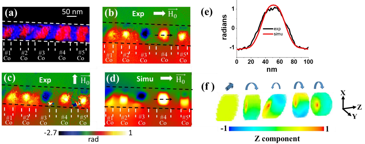
Figure 9: (a) EFTEM image of a 84 \pm 2 nm diameter Co_{50nm}/Cu_{50nm} nanocylinder. Experimental MPSI for H_s parallel (b) or perpendicular (c) to the wire axis and simulated MPSI (d) for H_s parallel to the wire axis. (e) Experimental (black) and simulated (red) amplitude of the MPSI at the position denoted by the dotted arrow in (b) and (d). (f) Corresponding 3D magnetic state for the 5 Co layers.
