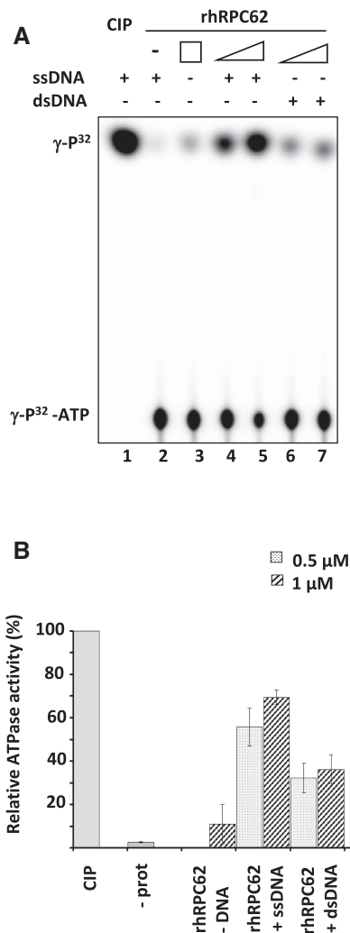
Figure 2. Characterization of rhRPC62 ATPase activity. (A) ATPase assays were conducted in presence of 0.5 \mu M of rhRPC62 (lanes 4, 6) or 1 \mu M of rhRPC62 (lanes 3, 5, 7). Lane 1: positive control with 1 unit of calf intestinal phosphatase (CIP); lane 2: negative control without protein. 2 \mu g of ssDNA were added to the reactions loaded in lanes 1, 2, 4 and 5. 2 \mu g of dsDNA were added to the reactions in lanes 6 and 7. (B) A quantification of three independent ATPase assays. \square : 0.5 \mu M protein, \square : 1 \mu M protein.
