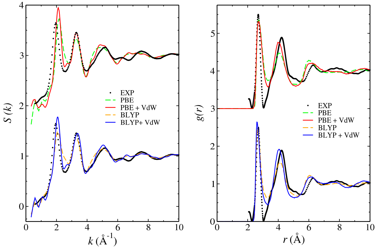
Figure 10: (Color online) Total structure factor S(k) (left panel) and pair correlation function (right panel) for \text{GeTe}_4 . FPMD models calculated using the BLYP functional (orange dashes) and the PBE (light green dashes) functional, as well as the BLYP + vdW (blue line) and PBE + vdW (red line) from Ref. 57, are shown in comparison with experimental data from Ref. 62.
