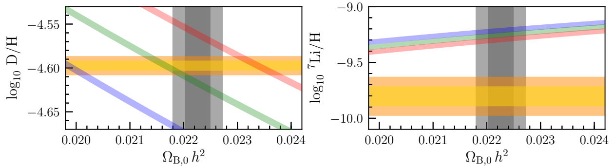
Figure 1: Measurements of (D/H)_P and ({}^7\text{Li}/H)_P (gold bands, left and right panels, respectively) compared to BBN calculations (coloured bands). The blue/green/red curves correspond to an effective number of neutrino species, N_{\text{eff}} = 2, 3, 4 , where the height of each band represents the uncertainty in the calculation. The Planck (2018) value of \Omega_{B,0} h^2 is shown by the gray band.
