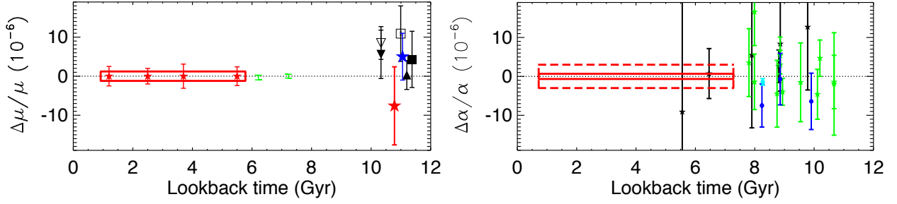
Figure 2: left: CJM comment: This caption is a bit confusing. Green points have different meanings in the two panels, and there is a high- z red point in the \mu panel which is not a POLLUX one. Existing \Delta\mu/\mu constraints (at high- z from \text{H}_2 and at intermediate- z from \text{NH}_3 and \text{CH}_3\text{OH} , green) compared with those expected for POLLUX observations (red points) of low- z \text{H}_2 systems. Combined POLLUX constraint, shown as red box, would be about an order of magnitude better than that of high- z \text{H}_2 system. right: The most precise existing \Delta\alpha/\alpha measurements (Murphy&Cooksey 2017) and the \Delta\alpha/\alpha precision expected from POLLUX shown as red dashed and solid boxes for individual and ensemble measurements, respectively. Both panels show the large empty gaps in the look-back time that would be covered by POLLUX.
