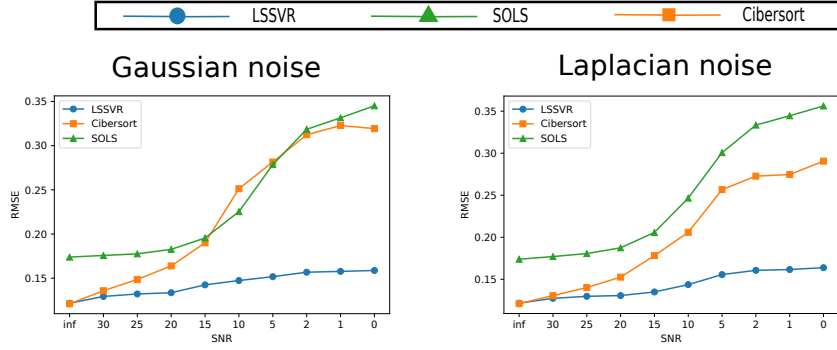
Fig. 4.2: The Root Mean Squared Error (RMSE) as a function of the Signal to Noise Ratio (SNR) is presented on a real dataset where noise was manually added. Two different noise distribution were tested: gaussian and laplacian. Each point of the curve is the mean RMSE of 12 different response vectors and we repeated the process four times for each level of noise. This would be equivalent to having 48 different repetitions.
