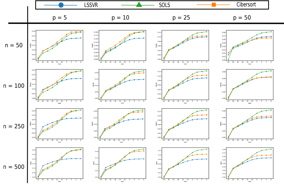
Fig. 4.1: The Root Mean Squared Error (RMSE) as a function of the Signal to Noise Ratio (SNR) is presented. Different dimensions for the design matrix X and the response vector y were considered. n represents the number of rows of X and p the number of columns. For each plot, the blue line represents the RMSE for the Linear Simplex SVR (LSSVR) estimator, the green one the Simplex Ordinary Least Squares (SOLS) estimator and the orange on the Cibersort estimator. Each point of the curve is the mean RMSE of 50 repetitions. The noise in the data has a gaussian distribution.
