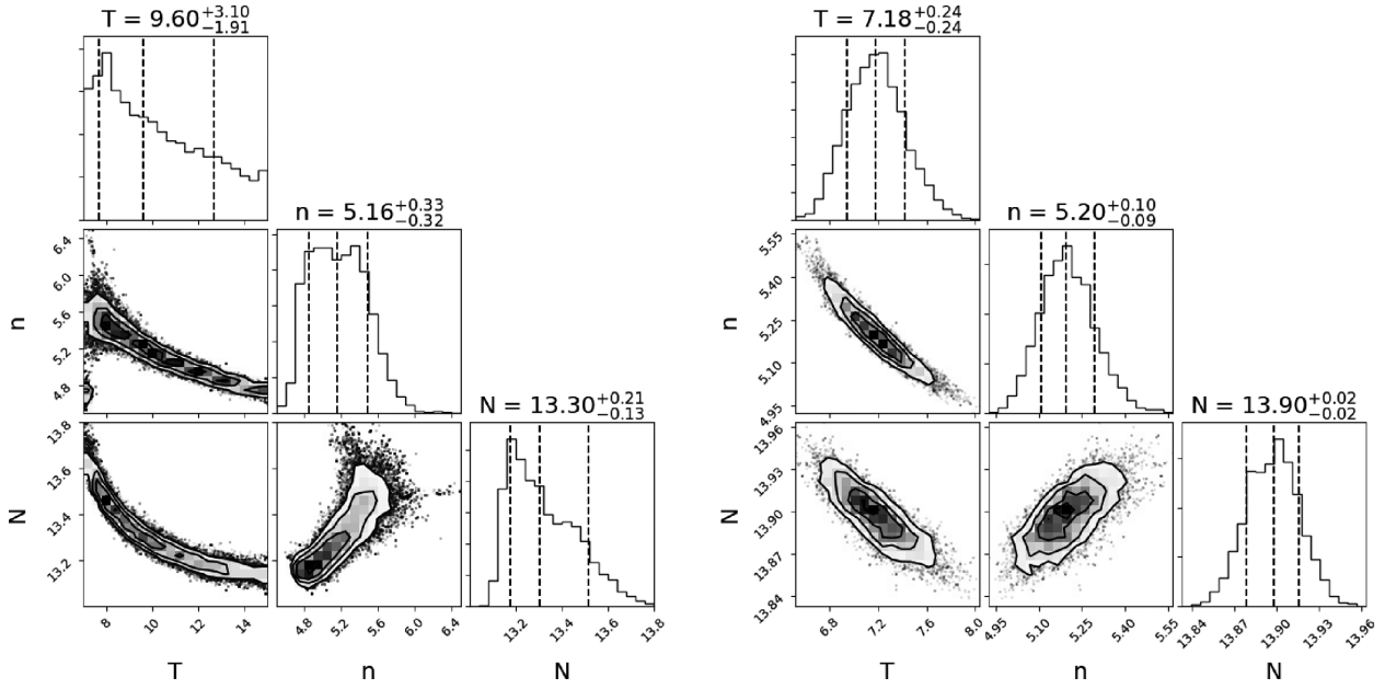
Figure 3. Histograms and cross-histograms from the MCMC parameter space exploration, for the kinetic temperature T , and for the \log_{10} of the density ( n ) and column density ( N ) of \text{HC}_3\text{N} derived from the rotational (left) and hyperfine (right) fluxes (see Table 1 and Section 3.4). In each histogram panel, the median value of the parameter, with the \pm 1\sigma boundaries (16 percent and 84 percent quantiles), are quoted and indicated by vertical dashed lines (see also Table 2).
