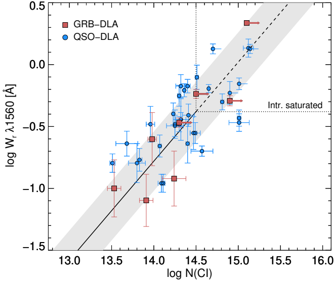
Fig. 7. \text{C I } \lambda 1560 rest-frame equivalent width as a function of total \text{C I} column density. Red squares denote GRB \text{C I} absorbers from this work. Blue dots show the \text{C I} -selected quasar absorbers from Ledoux et al. (2015), for which Noterdaeme et al. (2018) measured the total N(\text{C I}) from high-resolution spectroscopy. The black line shows the best linear fit where the \sigma = 0.3 dex scatter is shown by the gray-shaded region. The approximate column density (and equivalent width) at which the intrinsic \text{C I} lines saturate are marked by the dotted lines.
