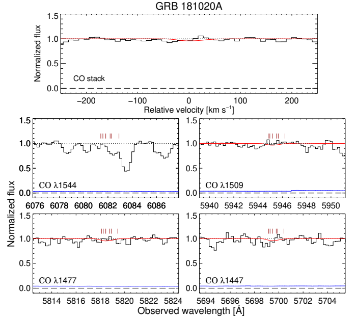
Fig. 8. Normalized VLT/X-shooter VIS arm spectrum of GRB 181020A showing the regions where the strongest CO band absorption lines are expected including a stacked spectrum (excluding \text{CO } \lambda 1544 ). Again, the solid black lines show the data and the blue lines the associated error. Line profiles showing the derived upper limits on N(\text{CO}) are overplotted in red.
