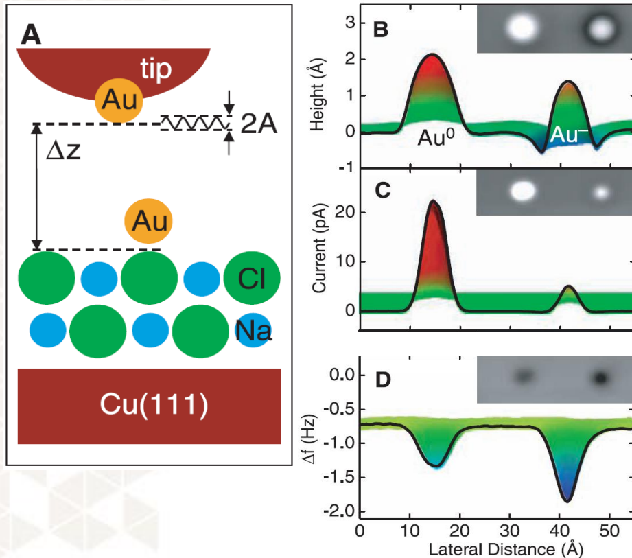
Spectroscopic sensitivity to the charge state on the atomic scale
