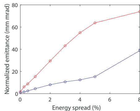
Figure 13. Simulated horizontal (red) and vertical (blue) normalized emittance of the electron beam at the undulator center for the low a_2 skew terms (Table 2) and the optics “slit-undulator” without slit using flat-top electron beams for different energy spread with 176 MeV central energy, \sigma'_{z,i} = 2 mrad, \sigma'_{x,i} = 3.12 mrad, and \epsilon_{z,i}, \epsilon_{x,i} = 0.2 mm.mrad.
