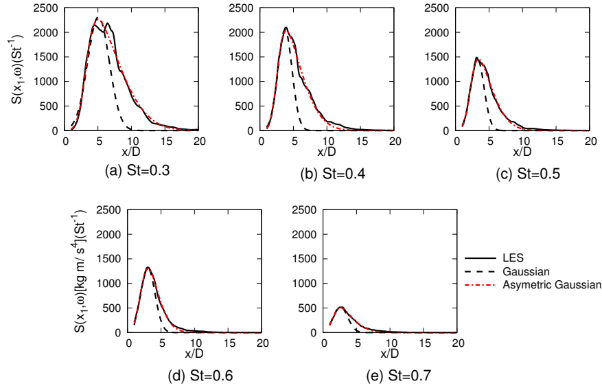
Figure 4: PSD of the source and fitted Gaussian and asymmetric envelopes.
