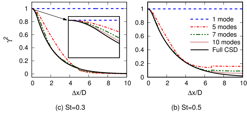
Figure 15: Coherence convergence of different low-rank approximations. Reference point is at x_0 .
