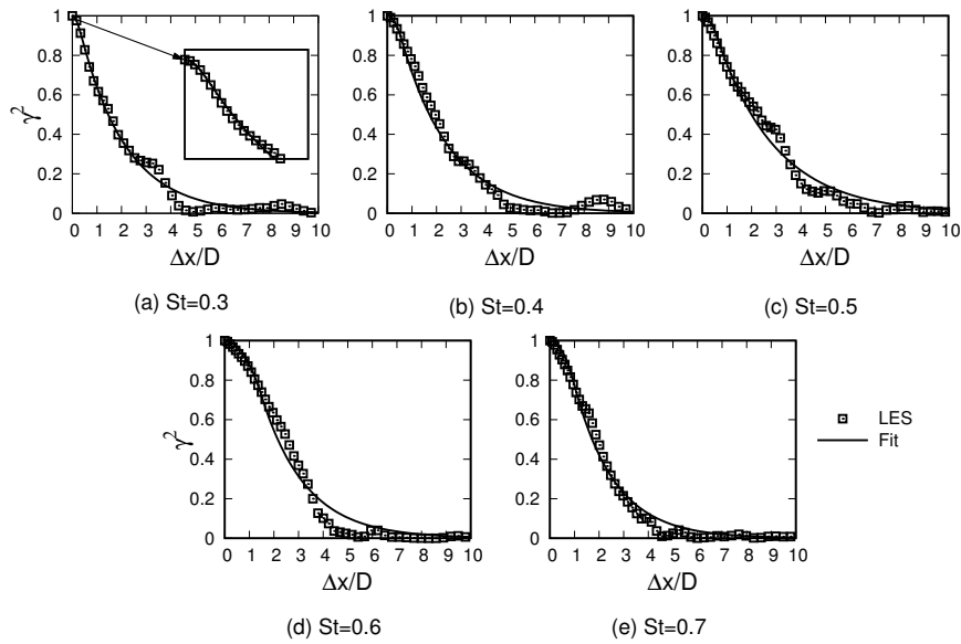
Figure 6: Magnitude-squared coherence of the LES data and fitted curves.
