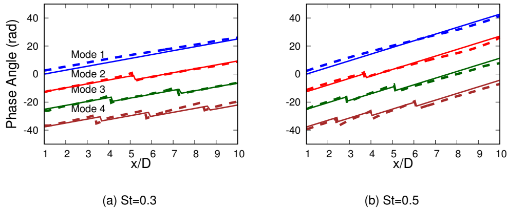
Figure 12: Phase of first 4 SPOD modes. Solid line represents the phases of the model CSD and dashed lines the phases of the CSD issued from LES data.
