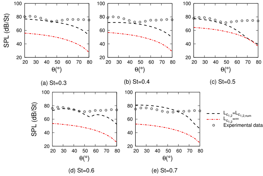
Figure 8: Comparison between sound radiated by single- and two-point wavepacket models and experimental data. The models have a Gaussian amplitude envelope.
