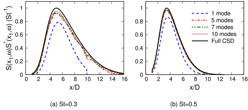
Figure 14: Wavepacket envelope convergence of different low-rank approximations. The levels have been normalised by the maximum value of the full source.
