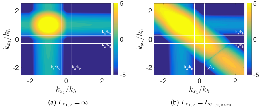
Figure 9: Fourier transform of CSD in wavenumber space at St=0.3 . (a): source with unit coherence; (b): source with coherence modulation. Levels are in dB scale.
