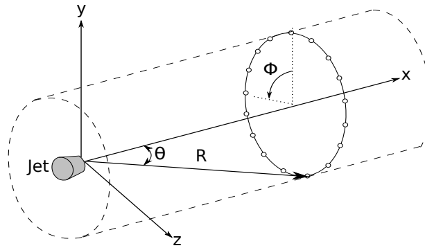
Figure 1: Schematic of microphone array.
