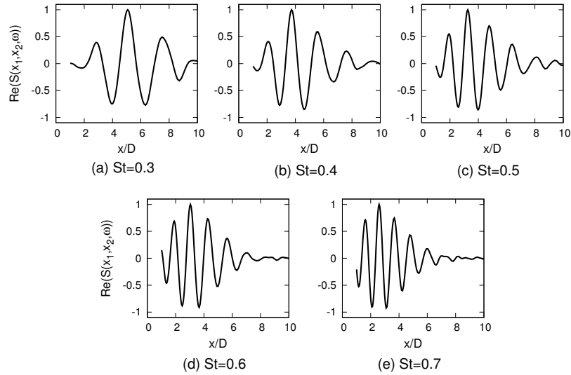
Figure 3: Radially-integrated CSD issued from the LES for different Strouhal numbers. Reference point is at x_0(\omega) . Levels have been normalised by the maximum value at each Strouhal number.
