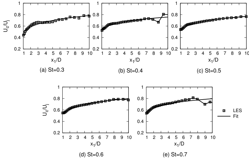
Figure 5: Phase velocity as a function of streamwise reference point, x_1 , for different Strouhal numbers and power-law fit.
