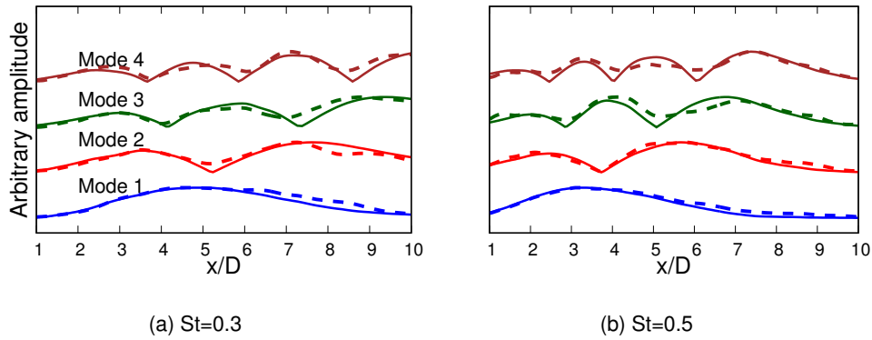
Figure 11: Structure of first 4 SPOD modes. Solid line represent the modes of the model CSD and dashed lines the modes of the CSD issued from the LES. The amplitudes are arbitrary and are in linear scale.
