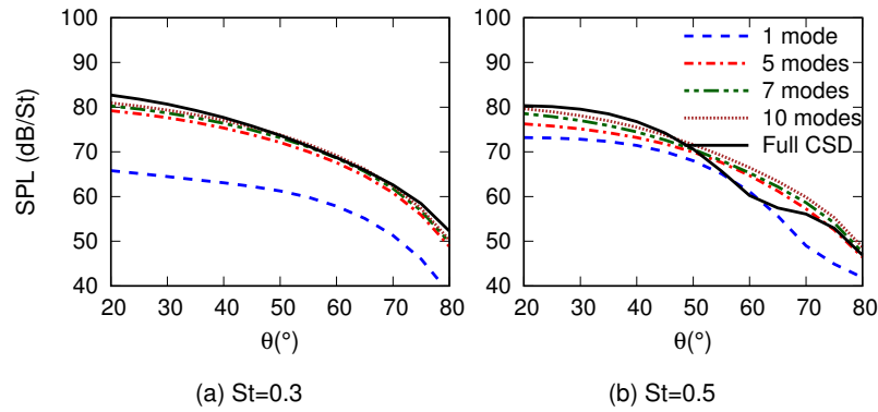
Figure 16: Effect of cumulative SPOD modes on far-field radiation by the wavepacket source.
