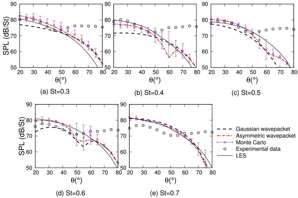
Figure 10: Sound radiation by sources with Gaussian and asymmetric amplitude envelopes. The error bars are centered at the mode of the sample values computed in the Monte Carlo simulation.
