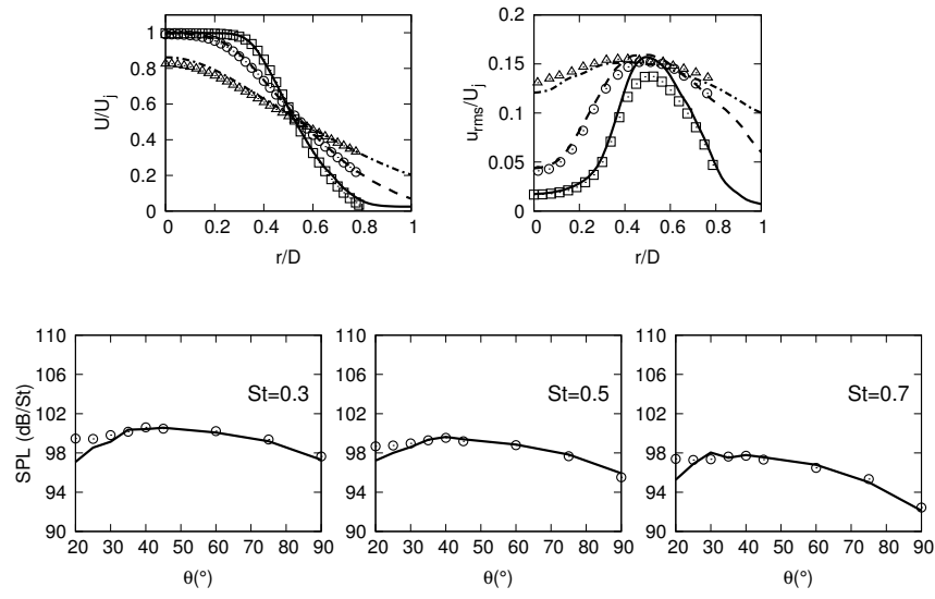
Figure 2: Top row: mean flow (left) and rms (right) radial profiles obtained from PIV (points) and LES (lines). Profiles at three streamwise stations are shown: x/D = 2.5 (solid line and squares); x/D = 4.5 (dashed-line and circles); x/D = 8 (dash-dotted-line and triangles). Bottom row: directivity plots for three Strouhal numbers with observer in the cylindrical surface delimited by the microphone array (figure 1). Circles: experimental data; solid line: LES far field prediction computed using the Ffowcs Williams & Hawkings equation.
