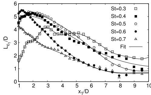
Figure 7: L_{c1} as a function of reference point for and polynomial fitting for various Strouhal numbers.
