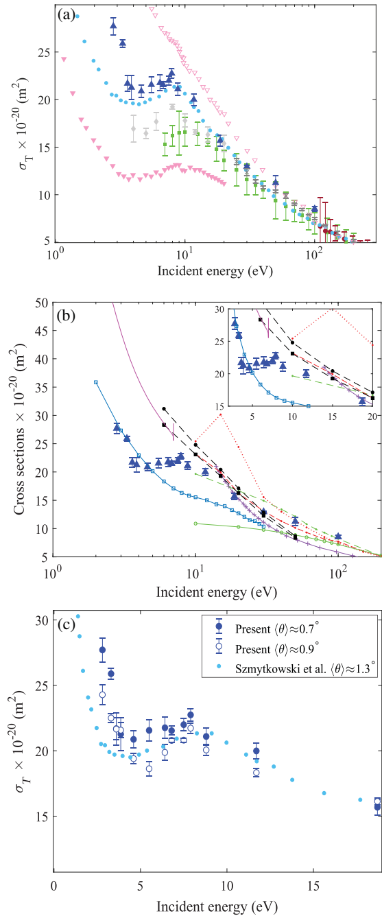
FIG. 3. (a) Total cross sections for electron scattering from H 2 O. Solid symbols correspond to direct measurements, hollow symbols to measurements corrected for forward-angle elastic scattering: filled triangle present results, cyan filled circle [30], filled inverted triangle [15], open inverted triangle [13], filled square [16], dark-red filled circle [31], times [32], filled rhombus [17]. (b) Total cross section comparison between present results filled triangle and theoretical predictions: dots SEP(CP)a1 [33], dotted dash SEP(ED)a1 [33]; integral elastic cross section dashed filled circle initial state J = 0 [34], and dashed filled square thermal average [34]; dash additivity rule [35], dashed open circle semiempirical formula [35], dashed open square Schwinger approach [36], solid line R matrix [37], dashed plus IAM plus BEB [30]. (c) Comparison among present \sigma_T for \langle \theta \rangle \approx 0.7^\circ and \langle \theta \rangle \approx 0.9^\circ , and results from Ref. [30].
