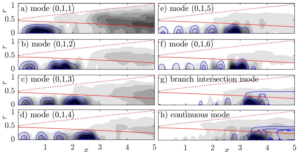
FIGURE 14. Same as figure 9 but comparing LES power spectral density estimate ( \square , 0 \leq \bar{P}_{pp}/\|\bar{P}_{pp}\|_{\infty} \leq 1 ) and the isolated trapped acoustic modes ( \|\hat{q}_m(x_0, r_0)\| \cdot \|\hat{q}_m^{\dagger}(x_0, r_0)\| , \blacksquare ). Contours of the product map correspond to 20%, 40%, 60%, and 80% of its maximum value.
