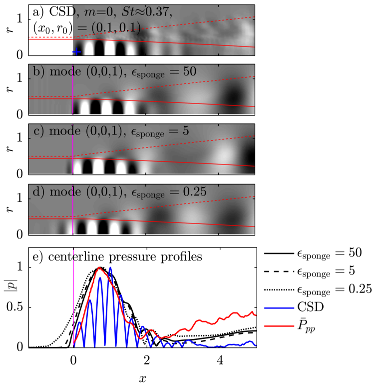
FIGURE 17. Influence of the sponge gain \epsilon_{\text{sponge}} on trapped acoustic modes and comparison with LES: (a) CSD of the LES as in 7(a); global modes with (b) \epsilon_{\text{sponge}} = 50 , (c) \epsilon_{\text{sponge}} = 5 , and (d) \epsilon_{\text{sponge}} = 0.25 ; (e) centerline pressure profiles. The same contour levels as in figure 7 are used in (a-d), and all profiles are normalized to unit maximum amplitude in (e). The LES PSD ( \bar{P}_{pp} , —) in (e) corresponds to the PSD along the axis in figure 9(a). The magenta line (—) indicates the beginning of the inlet sponge region in x < 0 .
