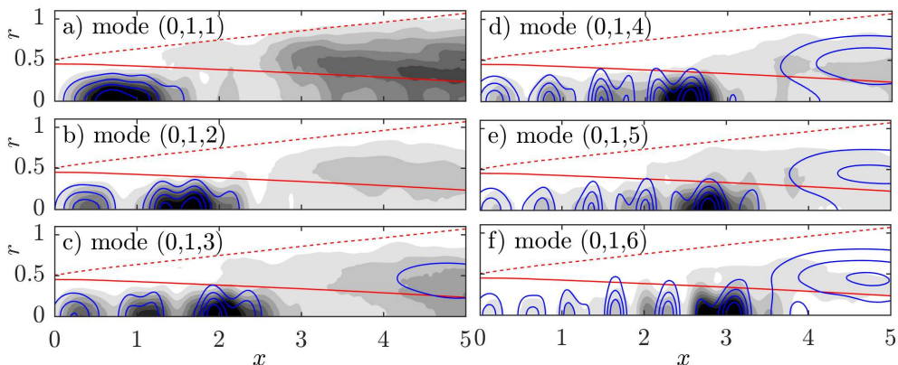
FIGURE 9. Comparison between the pressure components of LES power spectral density estimate ( \square \blacksquare , 0 \leq \bar{P}_{pp} / \|\bar{P}_{pp}\|_\infty \leq 1 ) and global mode ( \hat{p}_m \hat{p}_m^* , \blacksquare ) for branch (0,1) : (a) St \approx 0.374 , mode (0,1,1) ; (b) St \approx 0.382 , mode (0,1,2) ; (c) St \approx 0.39 , mode (0,1,3) ; (d) St \approx 0.397 , mode (0,1,4) ; (e) St \approx 0.405 , mode (0,1,5) ; (f) St \approx 0.41 , mode (0,1,6) . Contours of \hat{p}_m \hat{p}_m^* correspond to 20%, 40%, 60%, and 80% of its maximum value.
