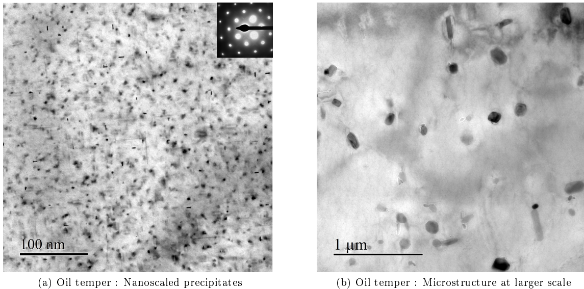
Figure 9: TEM pictures on oil temper
