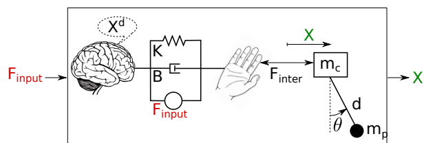
Fig. 1. Model used to analyze the dynamics of the task in simulation: Forward dynamics of the cart-and-pendulum system coupled to a model of hand impedance.
