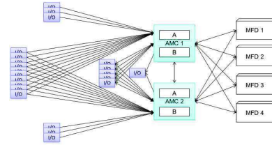
Figure 5: Vehicle Monitoring System
