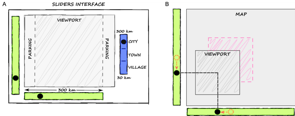
Fig. 6. (A) Sliders interface. For panning, users can move the viewport horizontally and vertically by moving two robots (black dots on the green areas) that represent the position of the viewport's center. Users can move the third robot in the zooming area (in blue) to select any scale between 30km and 300km. (B) Illustration of two successive sliders' and viewport's positions over the map.
