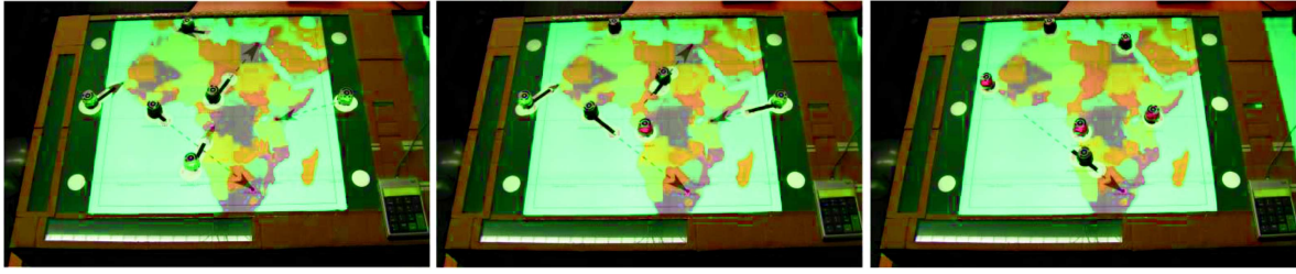
Fig. 7. Photographs illustrating how the robots move to reach their position by following lines displayed on the underlying screen. Arrows indicate the trajectories computed for each robot.
