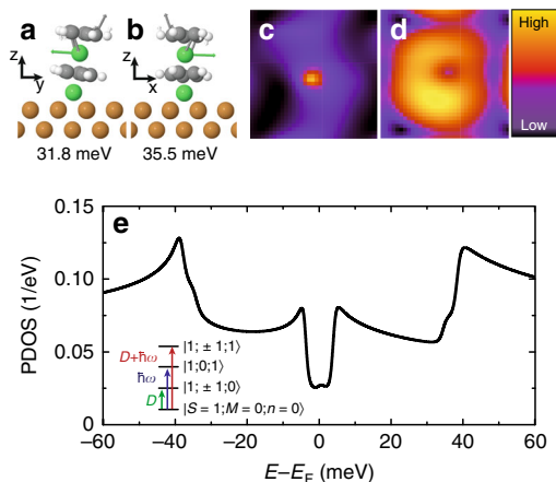
Fig. 3 Active vibrational modes and simulated spectrum of NiNc. a, b Calculated vibrational modes close to |\epsilon_2| . c Computed ratio between the inelastic and elastic tunneling conductance using the 35.5 meV mode. The maximum change represents 5% of the elastic conductance and is located in the center of the molecule. d Calculated local density of states of a NiNc complex at the Fermi level. e Projected density of states (PDOS) on the occupied molecular orbital as a function of electron energy calculated from Eq. (2). In the tunneling regime, the differential conductance is proportional to the PDOS 42 . Inset: State diagram of a NiNc complex based on Eq. (2); the eigenstates are noted as |S, M; n\rangle and the arrows depict the three transitions leading to the excitation steps in the dI/dV spectrum.
