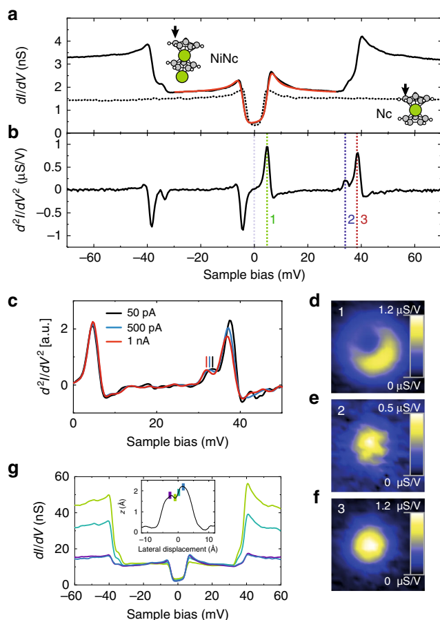
Fig. 2 Local spectroscopy of NiNc. a dI/dV spectrum and b d^2I/dV^2 spectrum acquired above the Cp ring of a NiNc complex (feedback loop opened at -80 mV and 200 pA). The solid red line is a fit based on a dynamical scattering model 34 . The data exhibited a negligible tip dependence as reflected by the measurement uncertainties over a collection of NiNc complexes. The energy onsets are labeled 1 , 2 , and 3 in b . The dashed curve in a is the dI/dV spectrum acquired above the Cp ring of a Nc in the layer (feedback loop opened at -70 mV and 100 pA). Inset: Arrow indicates the position where the spectrum was acquired. c d^2I/dV^2 spectra acquired above the center of a NiNc complex at various tip-molecule distances. The feedback loop was opened at 50 pA (solid black line), 500 pA (solid blue line) and 1 nA (solid red line) with a bias set to -20 mV—higher opening currents correspond to smaller tip-molecule distances. The spectra were normalized by the opening current. The vertical lines indicate the peak position of excitation 2 . d–f Spatial variation of the d^2I/dV^2 signal acquired at a constant-height and at a bias of 4.5 mV, 32.5 mV, and 37 mV, respectively (feedback loop opened at -60 mV and 500 pA above a Nc molecule of the layer; 3 mV rms modulation amplitude). These biases correspond to the excitation thresholds highlighted in b . g dI/dV spectra acquired at four locations above NiNc [indicated by colored dots in the line profile of NiNc presented in the inset]. The feedback loop was opened at -30 mV ( 300 pA) above all locations in order to have the same amplitude for step 1 in the dI/dV spectra.
