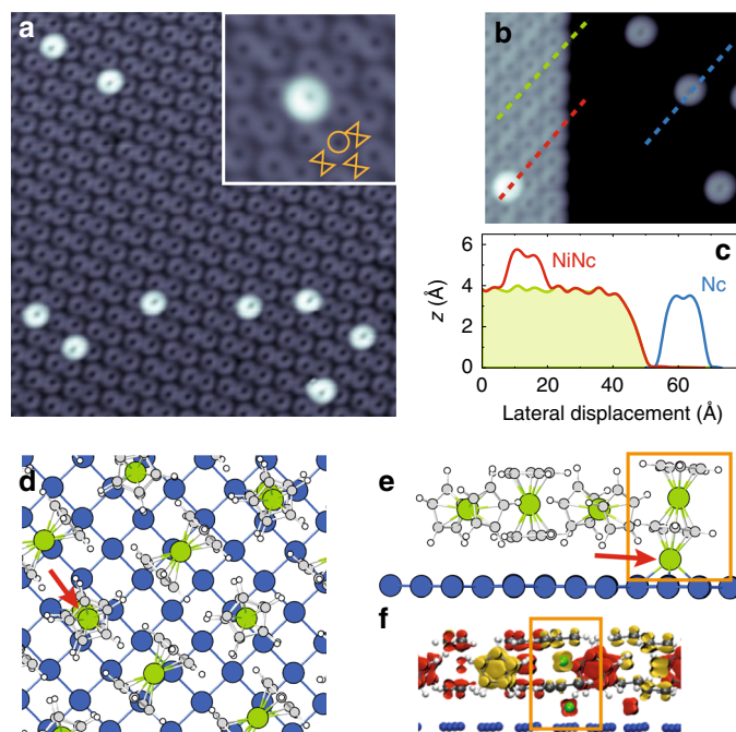
Fig. 1 NiNc adsorption in a nickelocene layer. a Self-assembled layer (paired configuration) and NiNc complex on Cu(100) (image size: 16 \times 16 nm 2 , sample bias: 20 mV, tunneling current: 20 pA). Inset: Close-up view of a NiNc complex in the paired layer. The molecular arrangement is sketched in orange as a circle for the vertical Nc and as a hourglass for the horizontal Nc ( 4 \times 4 nm 2 , 20 mV, 100 pA). b Edge of a paired layer and isolated Nc molecules on Cu(100) ( 10 \times 10 nm 2 , 20 mV, 100 pA) and c their corresponding height profiles along the dashed lines in b . d Top view, e side view of the DFT optimized structure of the NiNc complex embedded in a Nc paired layer—some molecules have been removed for clarity (H: white, C: gray, Ni: green). The red arrow indicates the position of the Ni adatom. f Side view of the spin density map of the paired structure containing two Ni atoms. Orange rectangles mark the NiNc complex. Yellow: Spin up, red: Spin down.
