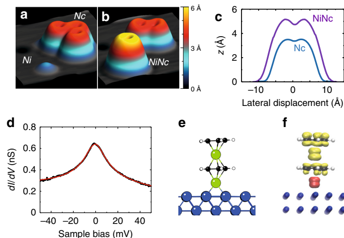
Fig. 4 Isolated NiNc on Cu(100). a, b Pseudo 3D images showing the tip-assisted assembly of an isolated NiNc complex ( 5 \times 5 \text{ nm}^2 , -20 \text{ mV} , 20 \text{ pA} ): a before and b after the transfer of Nc atop an isolated Ni adatom, and c height profiles of isolated NiNc and of isolated Nc. d dI/dV spectrum measured above the Cp ring of an isolated NiNc on Cu(100) (feedback loop opened at -50 \text{ mV} and 20 \text{ nA} ). The solid red line is a Frota-Fano fit yielding a resonance centered at -0.2 \pm 0.2 \text{ meV} and T_K = 68 \pm 7 \text{ K} . e DFT optimized structure of isolated NiNc on Cu(100), and f Side view of the spin density map.
