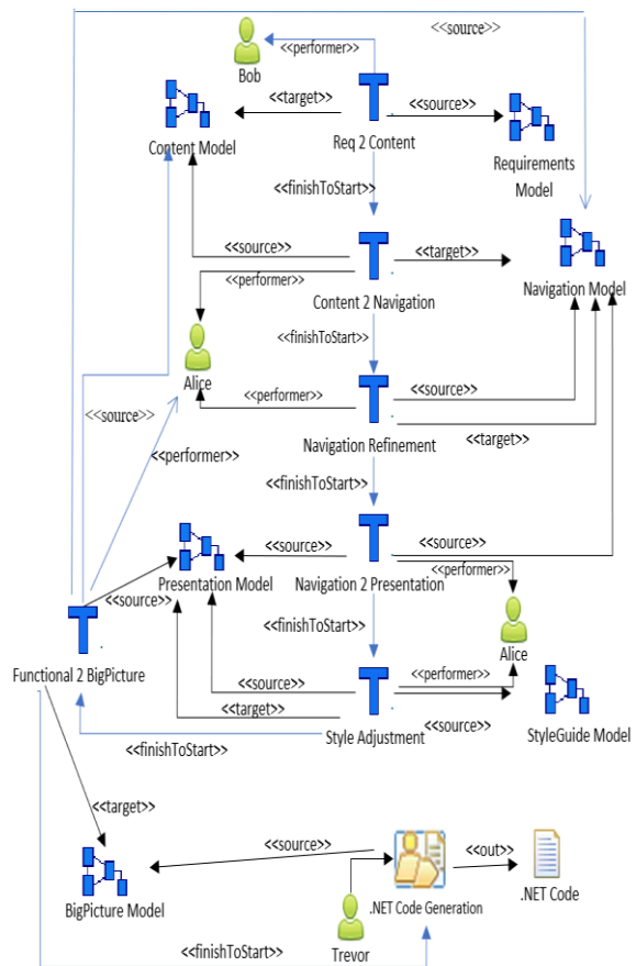
Figure 7: Enactable UWE Process Model.
