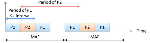
Fig. 2. Execution pattern
