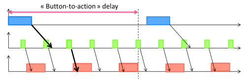
Fig. 3. Button-to-Action semantic
