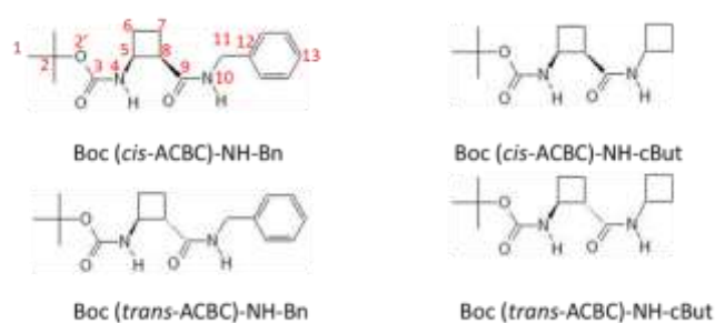
FIGURE 1 Molecules under study and numbering of atoms. \phi = \text{C}^3\text{-N}^4\text{-C}^5\text{-C}^8 \theta = \text{N}^4\text{-C}^5\text{-C}^8\text{-C}^9 \psi = \text{C}^5\text{-C}^8\text{-C}^9\text{-N}^{10} \psi_{\text{Ph}} = \text{C}^9\text{-N}^{10}\text{-C}^{11}\text{-C}^{12}
