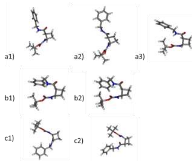
FIGURE 4 Structures of cis -ACBC (1 R ,2 S ) calculated at the B3LYP-D3/6-31G++(d,p) level of theory. a1) Mcis monomer as it is in the supramolecular structure (see text) a2) Mcis monomer optimised without dispersion a3) Mcis monomer optimised with dispersion b1) c-1 structure evidenced in the gas phase, with a C8 intramolecular hydrogen bond, optimised without dispersion b2) same with dispersion c) c-3 structure evidenced in the gas phase, with a C6 intramolecular hydrogen bond optimised without dispersion, c2) same with dispersion.
