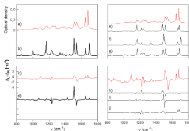
FIGURE 3 Left: a) Experimental IR absorption of cis -ACBC (1 R ,2 S ) (red) b) calculated IR absorption of the monomer subunit Mcis c) Experimental VCD spectrum of (1 R ,2 S ) (red) d) calculated VCD spectrum of the monomer subunit (see text). Right: Experimental IR absorption of cis -ACBC (1 R ,2 S ) (red) and calculated IR absorption of e) c-1 f) c-3 g) c-2 . e) Experimental VCD spectra of cis -ACBC (1 R ,2 S ) (red) and calculated VCD spectrum of h) c-1 i) c-3 j) c-2 . The calculations are at the B3LYP /6-31G++(d, p) level. The harmonic frequencies are scaled by 0.97.
