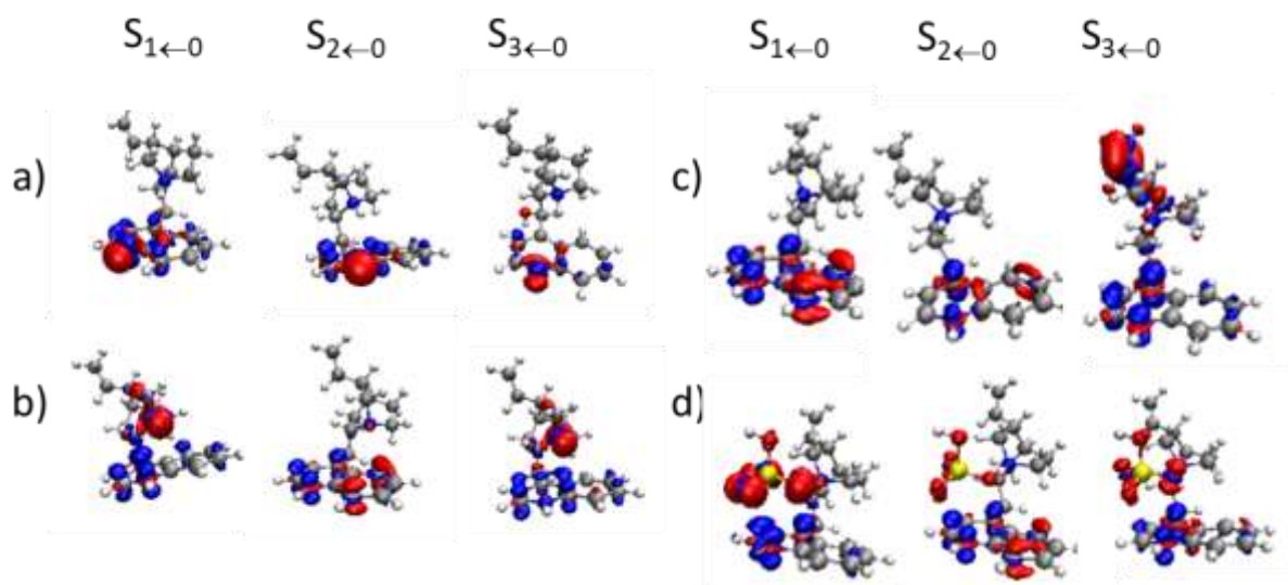
Figure 11: Difference between the electronic density of the ground state and that of the first three excited states. The isolvalue is set to 0.005. The red (blue) color codes a decrease (increase) in electron density, respectively: a) \text{CdH}^+ , with the proton located on N_{\text{alk}} b) \text{CdN}_{\text{arom}}\text{H}^+ , with the proton located on N_{\text{arom}} c) \text{CdH}_2^{2+} with N_{\text{alk}} and N_{\text{arom}} protonated d) \text{CdH}_2^{2+}\text{HSO}_4^- complex.
