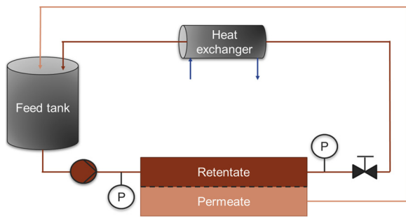
Fig. 1. Set-up of the filtration system used for the screening of membranes for the filtration of sugarcane bagasse mild alkaline extract.
