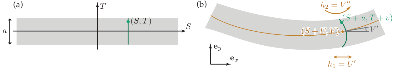
Figure 5: A block of a linearly elastic material in (a) reference and (b) current configuration. The 1d model makes use of the center line (brown curve), defined as the curve passing through the centers of mass (brown dots) of the cross-section. The macroscopic strain are the apparent stretch h_1(S) = U'(S) and the apparent curvature h_2(S) = V''(S) of the center line.
