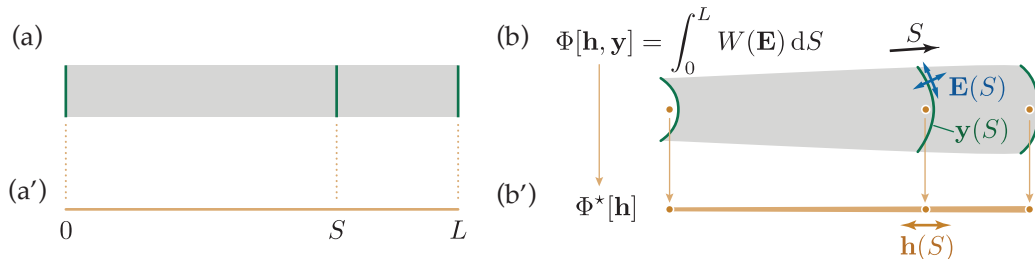
Figure 1: Dimension reduction for an abstract slender structure. Left column (a,a') : reference configuration highlighting a particular cross-section with coordinate S . Right-hand side column (b,b') : deformed configuration. Top row (a,b) : full model used as a starting point, including a microscopic displacement \mathbf{y}(S) and a microscopic strain \mathbf{E}(S) . Bottom row (a',b') : equivalent 1d model obtained by dimension reduction, in which the details at the scale of cross-section are effectively hidden.
