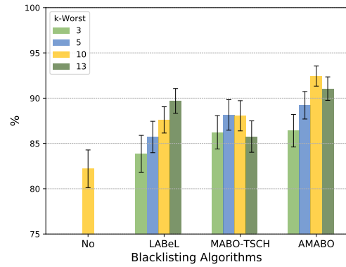
Fig. 6: Link-level Packet Delivery Ratio.
