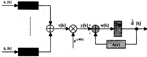
Fig. 3. SOC-MI-DFE (tracking mode).
