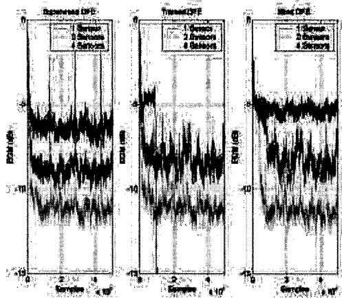
Fig. 4. Evolution of MSE for supervised, trained and blind spatio-temporal DFE (4-PSK).
