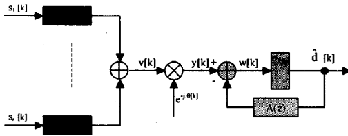
Fig. 3. SOC-MI-DFE (tracking mode).
