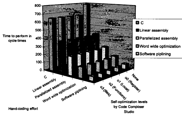
Fig. 7. Hand-coding effort vs. CCS self-optimization . Time to perform a 20 taps FIR filtering.
