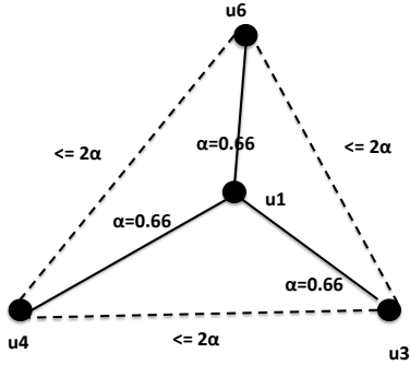
Fig. 4: An instantiation of \text{GrpDia}(0.66) using the example in Section 2. The clique involving u_1, u_3, u_4, u_6 can not have an edge with distance > 2 \times 0.66 , due to the triangle inequality property.
