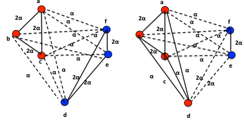
Fig. 5: Balanced Partitioning in SpltB0pt when the distance satisfies triangle inequality for a graph with 6 modes. The left hand side figure has two partitions ( \{a, b, c\}, \{d, e, f\} ) with 3-nodes in each (red nodes create one partition and blue nodes create another). The intra-partition edges are drawn solid, whereas, inter-partition edges are drawn as dashed. Assuming K = 4 , in the right hand side figure, node d is moved with a, b, c . This increases the overall inter-partition weights, but is bounded by a factor of 2.
