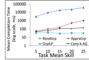
Fig. 17: Grp : Mean Completion Time varying Mean Skill
