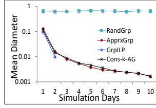
Fig. 14: Grp : Mean Diameter varying Simulation Days
