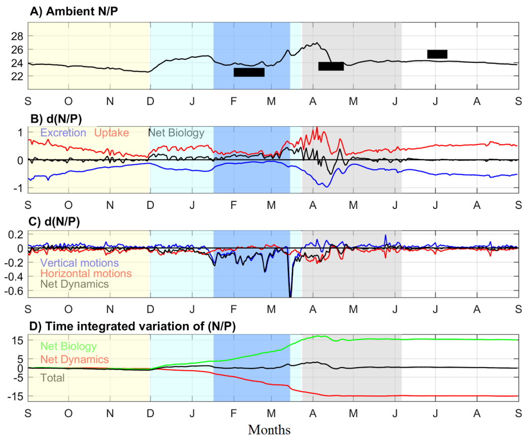
730 Figure 11. (A) Time series of the modeled N:P ratio ( \text{molN molP}^{-1} ) averaged in the upper layer 731 [0-130 m] of the Deep Convection Area from September 2012 to September 2013. Estimates 732 from observations are shown as horizontal bars overlaying the model output. (B) 733 Biogeochemical and (C) physical processes ( \text{molN molP}^{-1} \text{d}^{-1} ) influencing the N:P dynamics and 734 (D) their net time integrated resultant.
