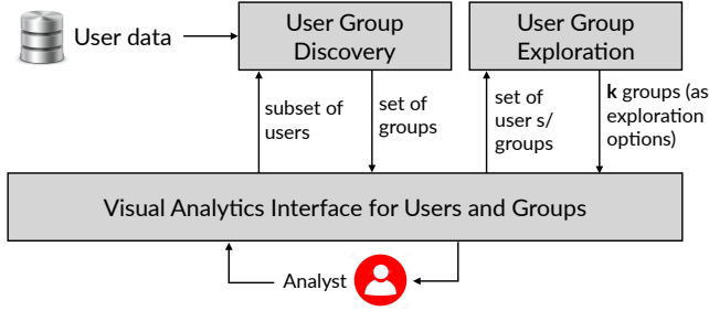
Figure 1: UserDEV architecture.
