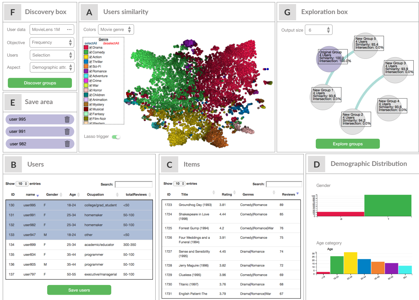
Figure 2: UserDEV visual interface displaying the MovieLens dataset.
