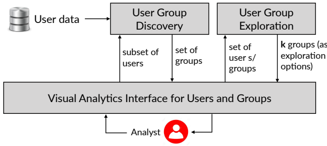
Figure 1: UserDEV architecture.
