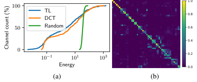
Fig. 3: (a): Cumulative distribution of the atoms contributing energies for three transforms \Phi . (b): Similarity matrix between the 50 most-contributing atoms learnt from two different random initializations.
