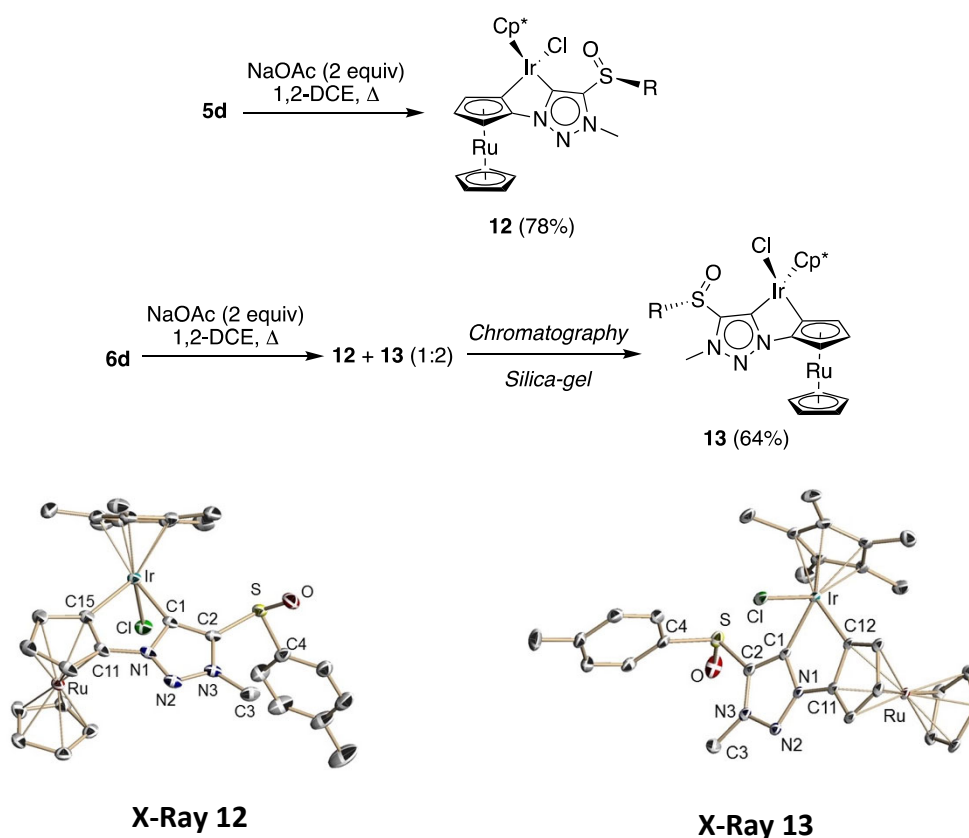
Scheme 8. The stereodivergent synthesis of enantiopure planar-chiral bimetallic ruthenacycles 12 and 13 . Selected bond lengths [ \text{\AA} ] and angles [ ^\circ ] for 12 : Ir-C1 2.013(4), Ir-C15 2.066(4), Ir-Cl 2.425(1), C1-C2 1.383(6), C2-N3 1.371(5), N1-N2 1.322(5), N2-N3
