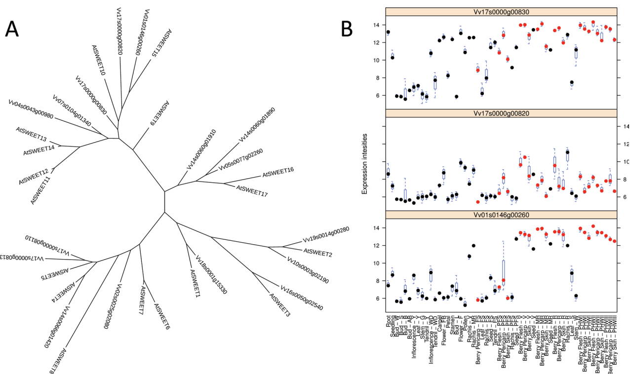
Fig. 1. Phylogenetic tree and berry expression of SWEET transporter genes in grape. (A) Evolutionary tree of grapevine and Arabidopsis SWEET transporters inferred by using the maximum likelihood method implemented in the MEGA5 software (Tamura et al. , 2011). Grapevine SWEET were identified by their PFAM (Punta et al. , 2012) domain PF03083. (B) Boxplot of gene expression profiles over a microarray developmental series made by Fasoli et al. (2012) for the three most berry-specific VvSWEET genes: Vv01s0146g00260, Vv17s0000g00820, and Vv17s0000g00830. Red dots indicate median expression intensities for berry samples. Data were obtained from NCBI GEO (Barrett et al. , 2013; accession no. GSE36128) and RMA normalized using the R/oligo package (Carvalho and Irizarry, 2010).
